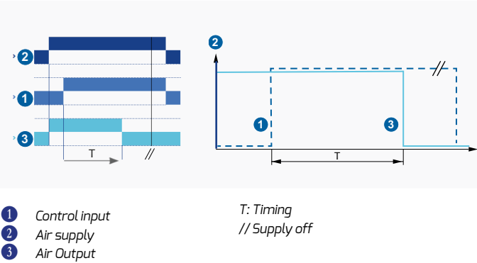
Negative Output
