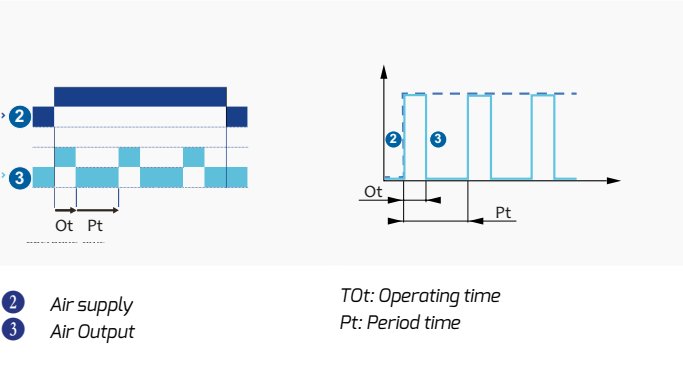
Frequency Generator
