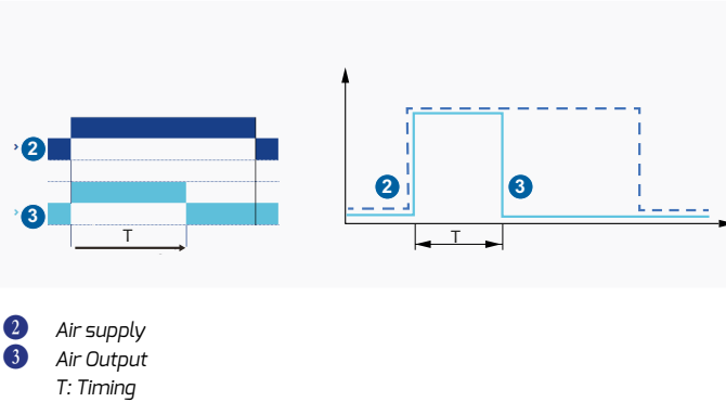
Impulse Generator
